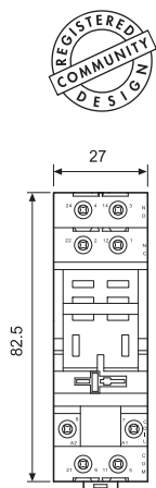
96.02
